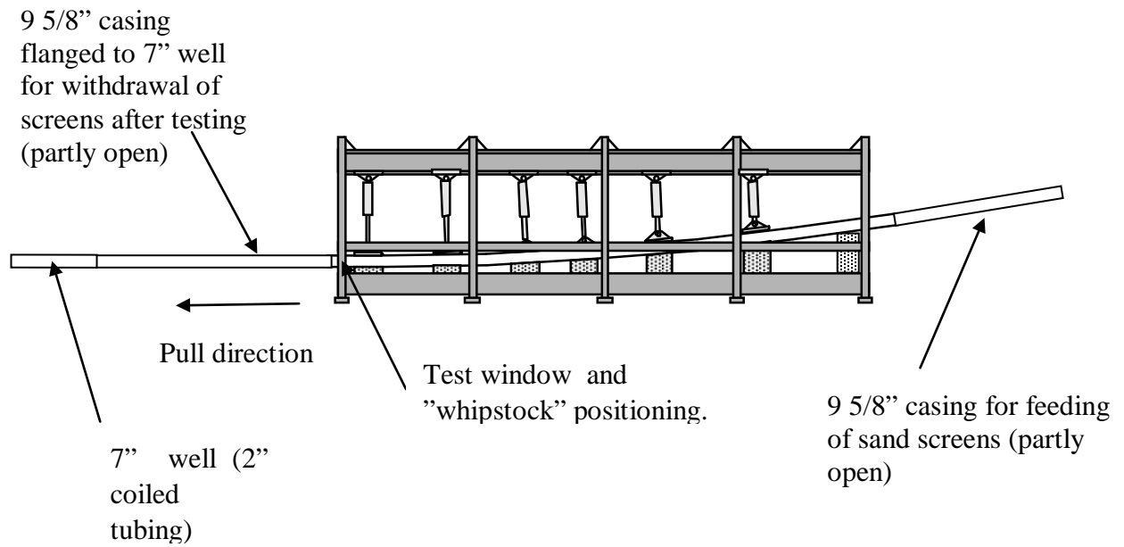
Hydraulic test frame
